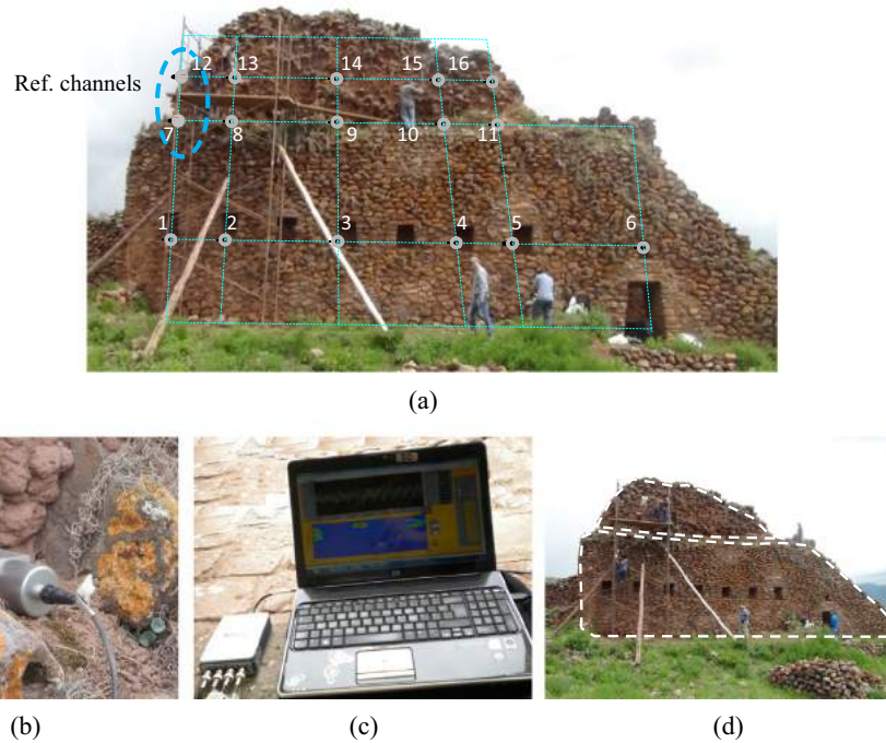
Fig. 3. OMA tests at Chokepukio: (a) test setup, (b) close up of a measurement node, (c) central acquisition station and (d) general view of the instrumented wall and the process of fixing sensors.
